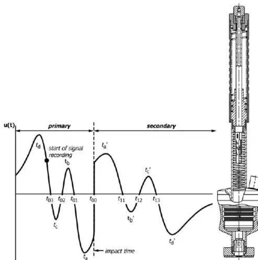
FIG. X2.2 Design of the Kraukramer Impact Device D
